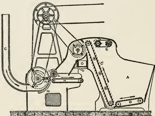
COTTON OPENER AND PICKER
